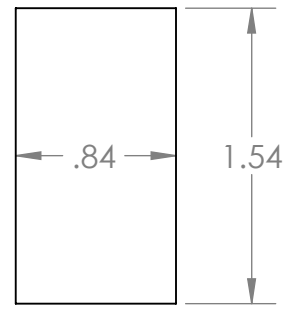
Dash Mount Installation Template
